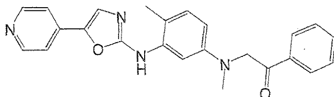
10 030: 2-{Methyl-[4-methyl-3-(5-pyridin-4-yl-oxazol-2-ylamino)-phenyl]-amino}-1-phenyl-ethanone
