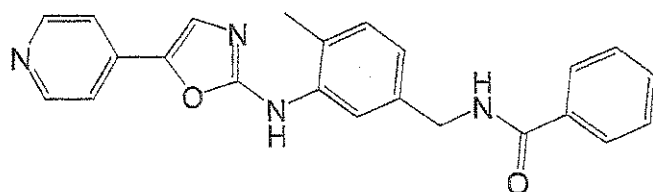
029: N-[4-Methyl-3-(5-pyridin-4-yl-oxazol-2-ylamino)-benzyl]-benzamide
