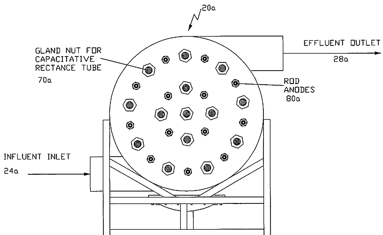
FIG. 7 END VIEW OF ELECTROLYTIC CELL
