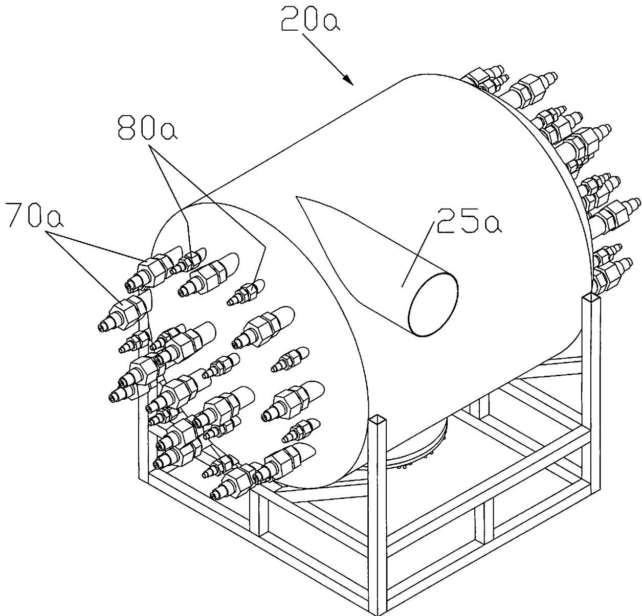
FIG. 4 ELECTROLYTIC CELL
