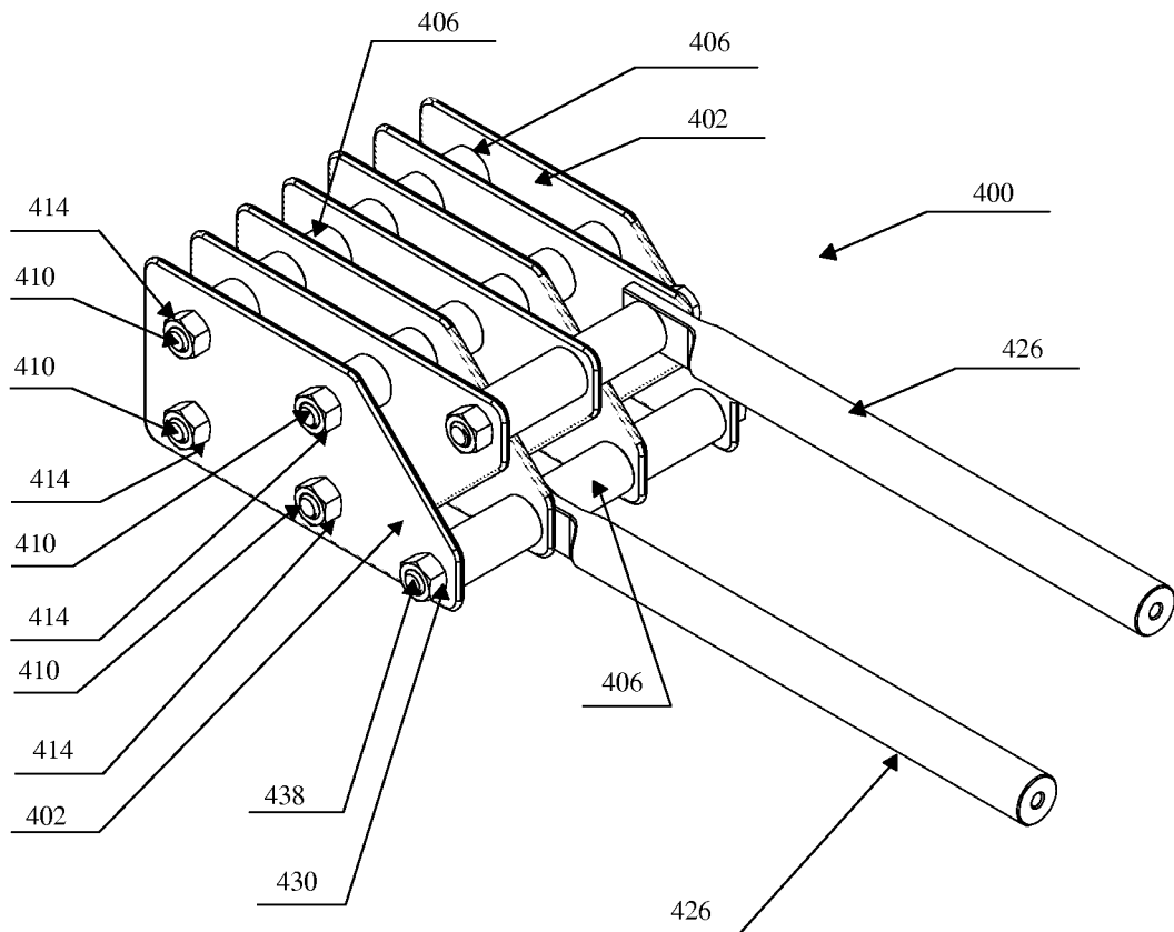
FIGURE 11: OVER ALL LOOK OF NOVEL ELECTRO CATALYTIC PADDLE ELECTRODE
