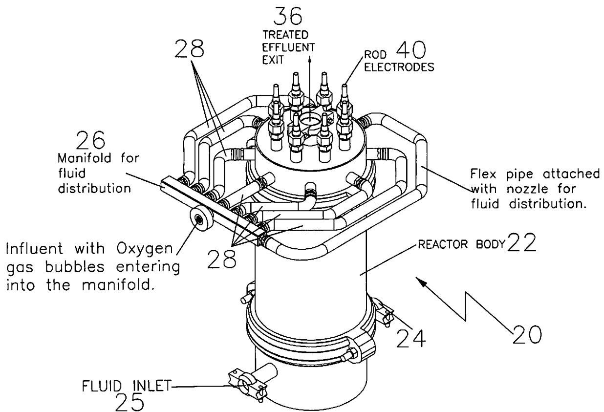
FIG. 1 ELECTRO-CHEMICAL CELL REACTOR
