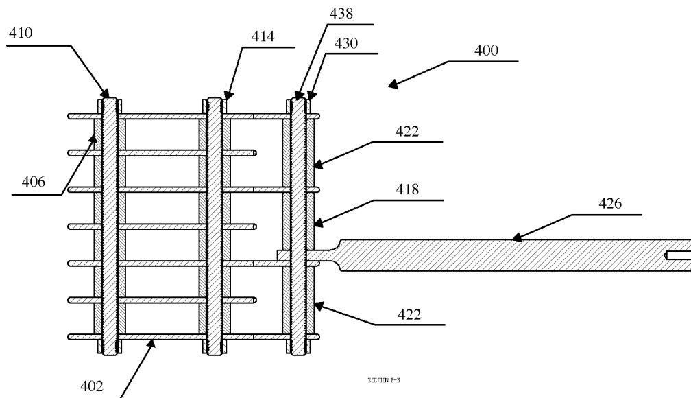
FIGURE 12: DETAILED CONSTRUCTION OF THE NOVEL ELECTRO -CATALYTIC PADDLE ELECTRODE
