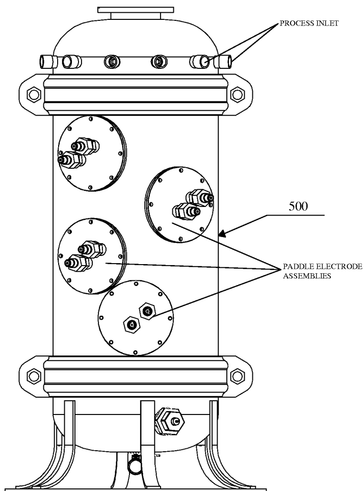
ELECTRO-CATALYST REACTOR WITH PLATE TYPE PADDLE ELCTRODES
