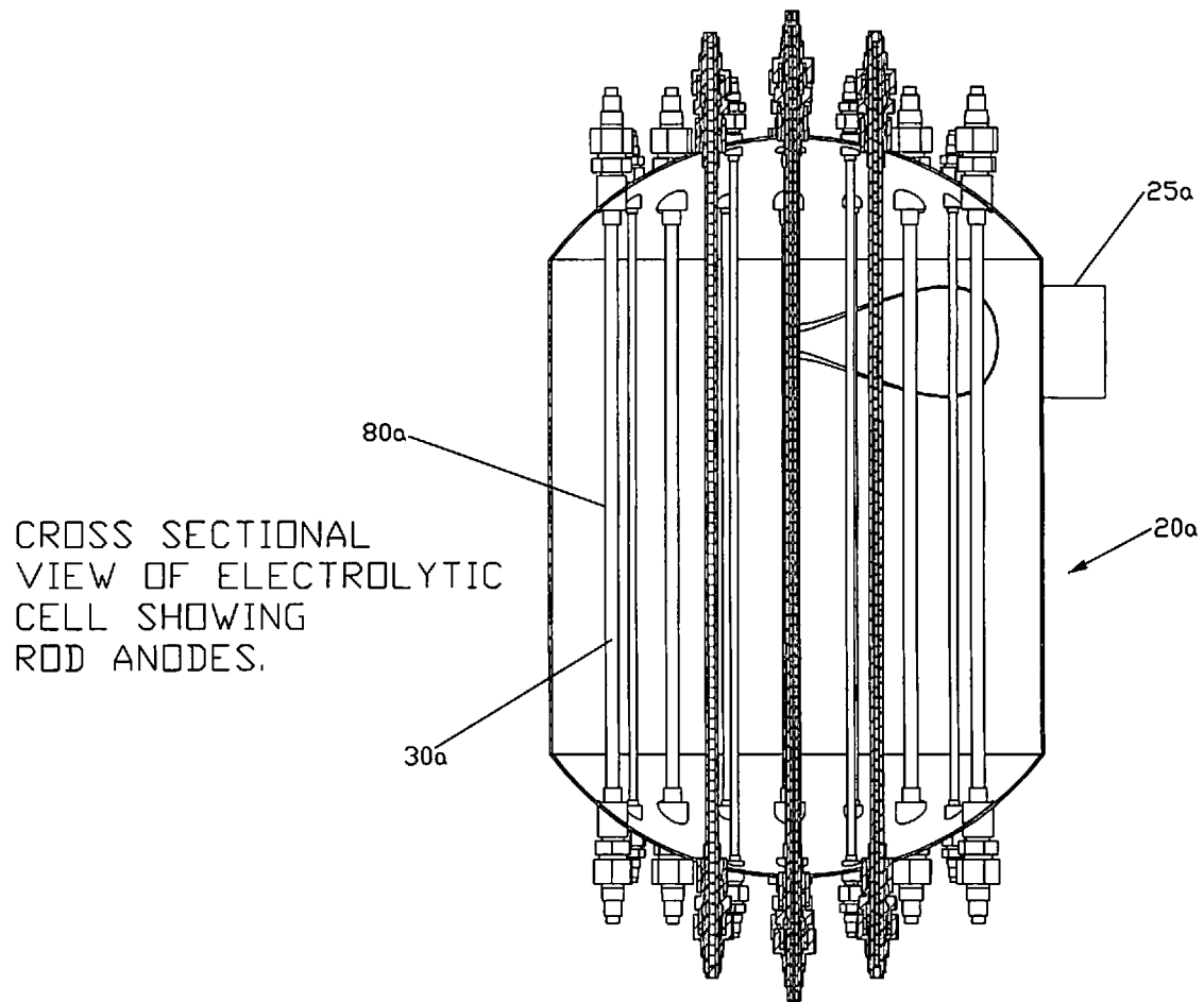
FIG.6 TOP CROSS SECTIONAL VIEW OF ELECTRO-CHEMICAL CELL.
