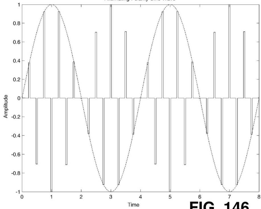
Alternating Polarity Sine Wave
