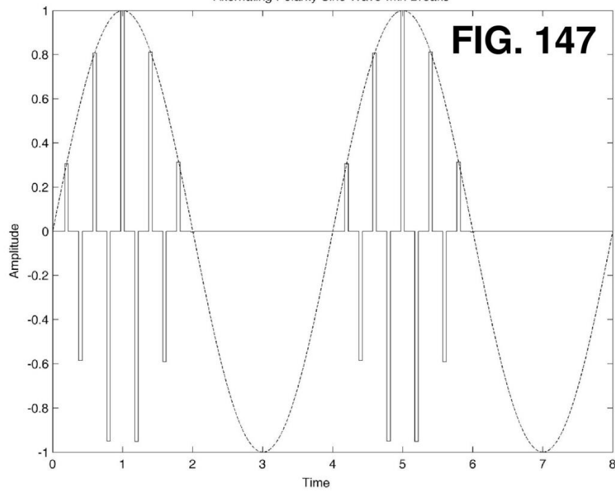
Alternating Polarity Sine Wave with Breaks
