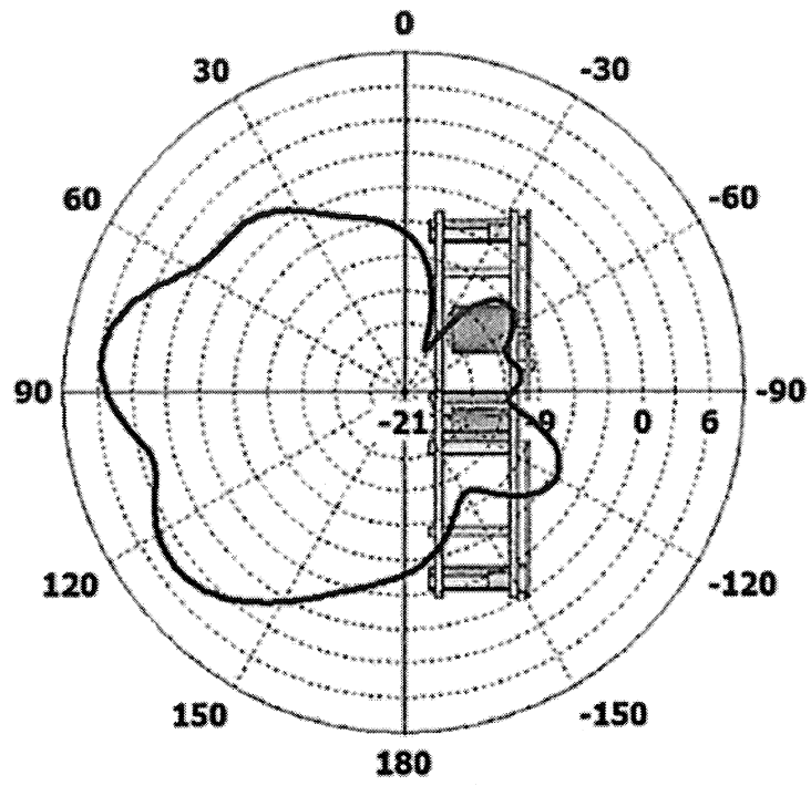
Phi / Degree vs. dBi
