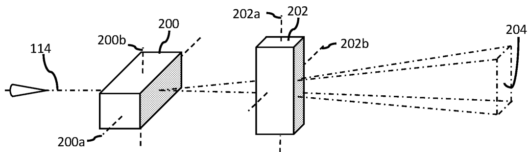
FIG. 2 (RELATED ART)
