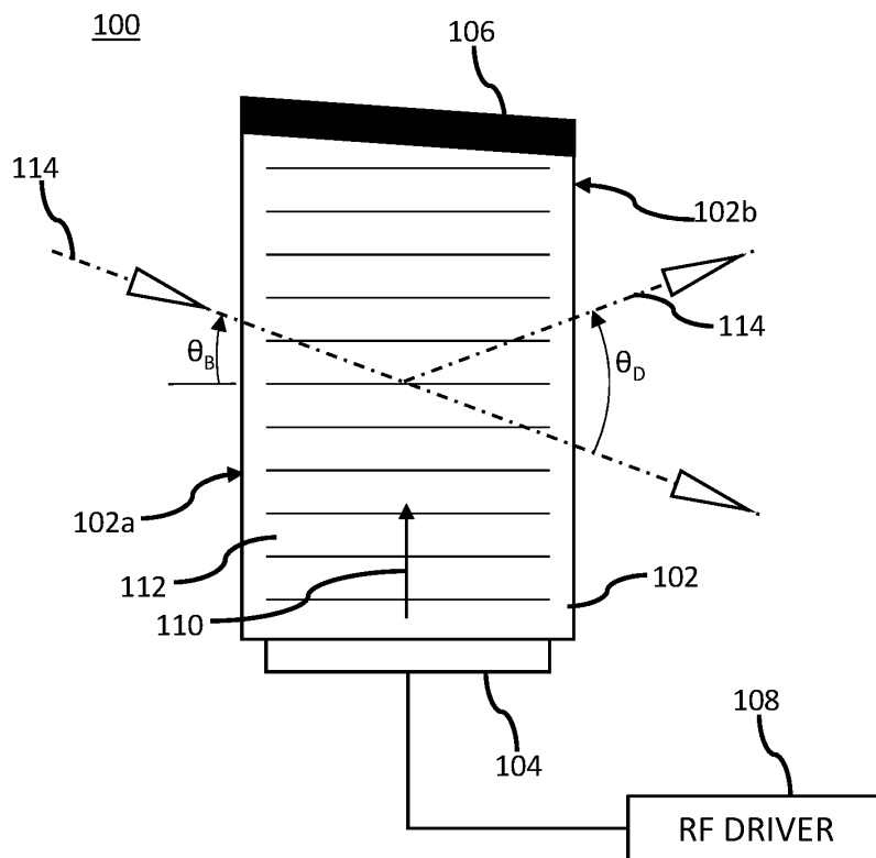
FIG. 1 (RELATED ART)
