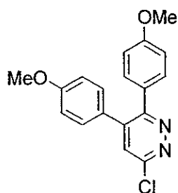
Comparative Compound 1
