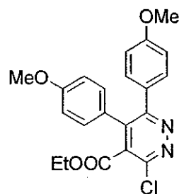
Comparative Compound 2
