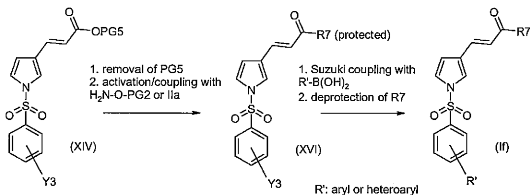
Reaction scheme 7:
