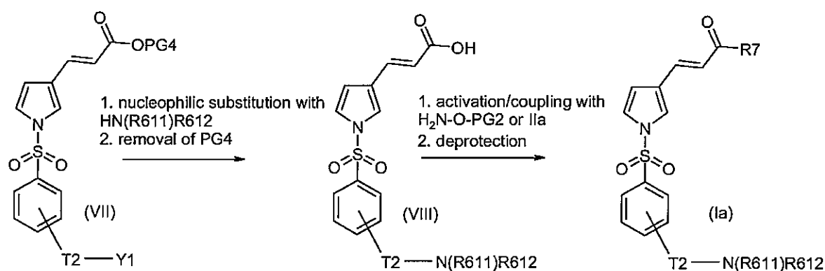
Reaction scheme 2:
