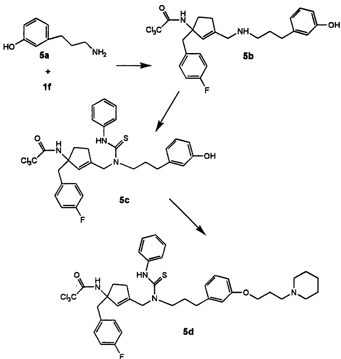
Scheme 5
