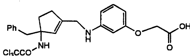
Cpd 45
