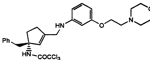
Cpd. 6b
