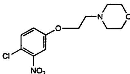
Compound 35
