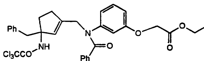
Cpd 46
