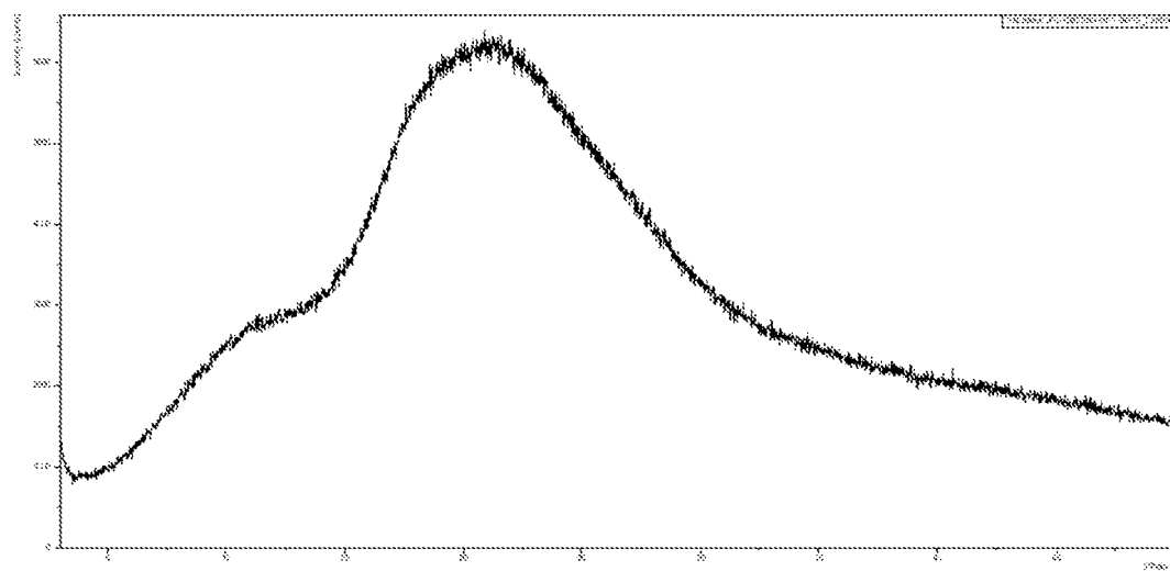
Figure 9. PXRD
