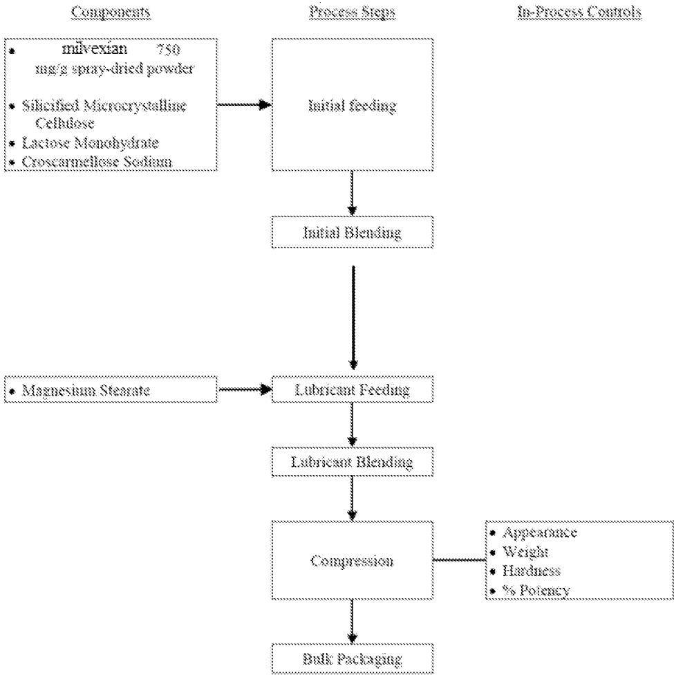
Figure 1: Flowchart of Manufacturing Process for the milvexian 25 mg oral tablet and 100 mg oral tablet
