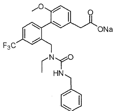
(Compound 2).
