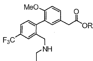
Formula V
