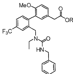
Formula VI;
