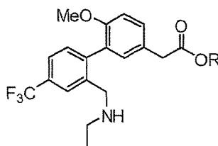
Formula V
