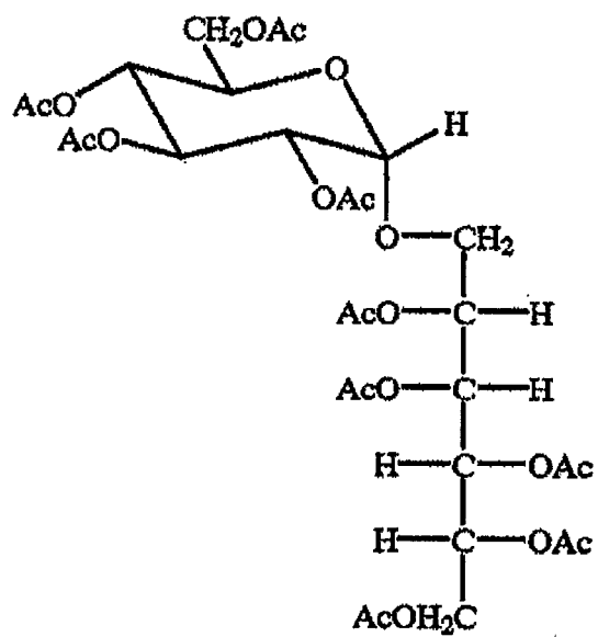
GPM nonaacetate ( \alpha -D-glucopyranosyl-1 \rightarrow 6-mannitol nonaacetate)
