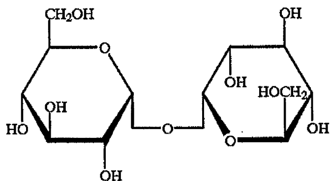
Trehalose ( \alpha -D-Glucopyranosyl- \alpha -D-glucopyranoside)
