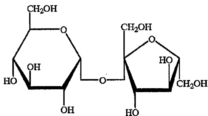
Sucrose ( \alpha -D-glucopyranosyl- \beta -D-Fructofuranoside)
