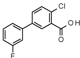
2-Chloro-5-(3-fluorophenyl)benzoic acid (intermediate III(g))
