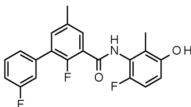
2-Fluoro-N-(6-fluoro-3-hydroxy-2-methyl-phenyl)-3-(3-fluorophenyl)-5-methyl-benzamide
