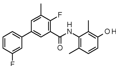
2-Fluoro-5-(3-fluorophenyl)-N-(3-hydroxy-2,6-dimethyl-phenyl)-3-methyl-benzamide
