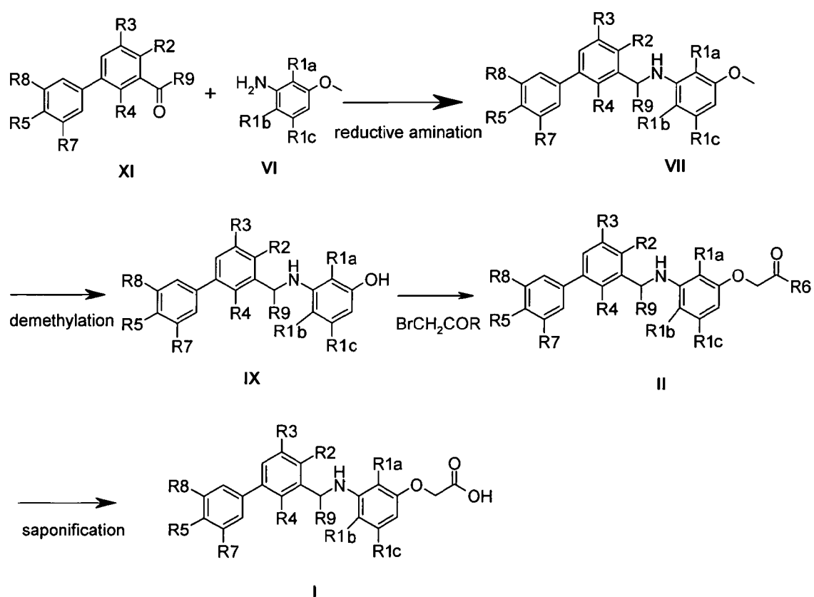
Scheme 5:
