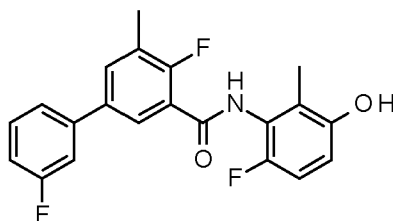
2-Fluoro-N-(6-fluoro-3-hydroxy-2-methyl-phenyl)-5-(3-fluorophenyl)-3-methyl-benzamide
