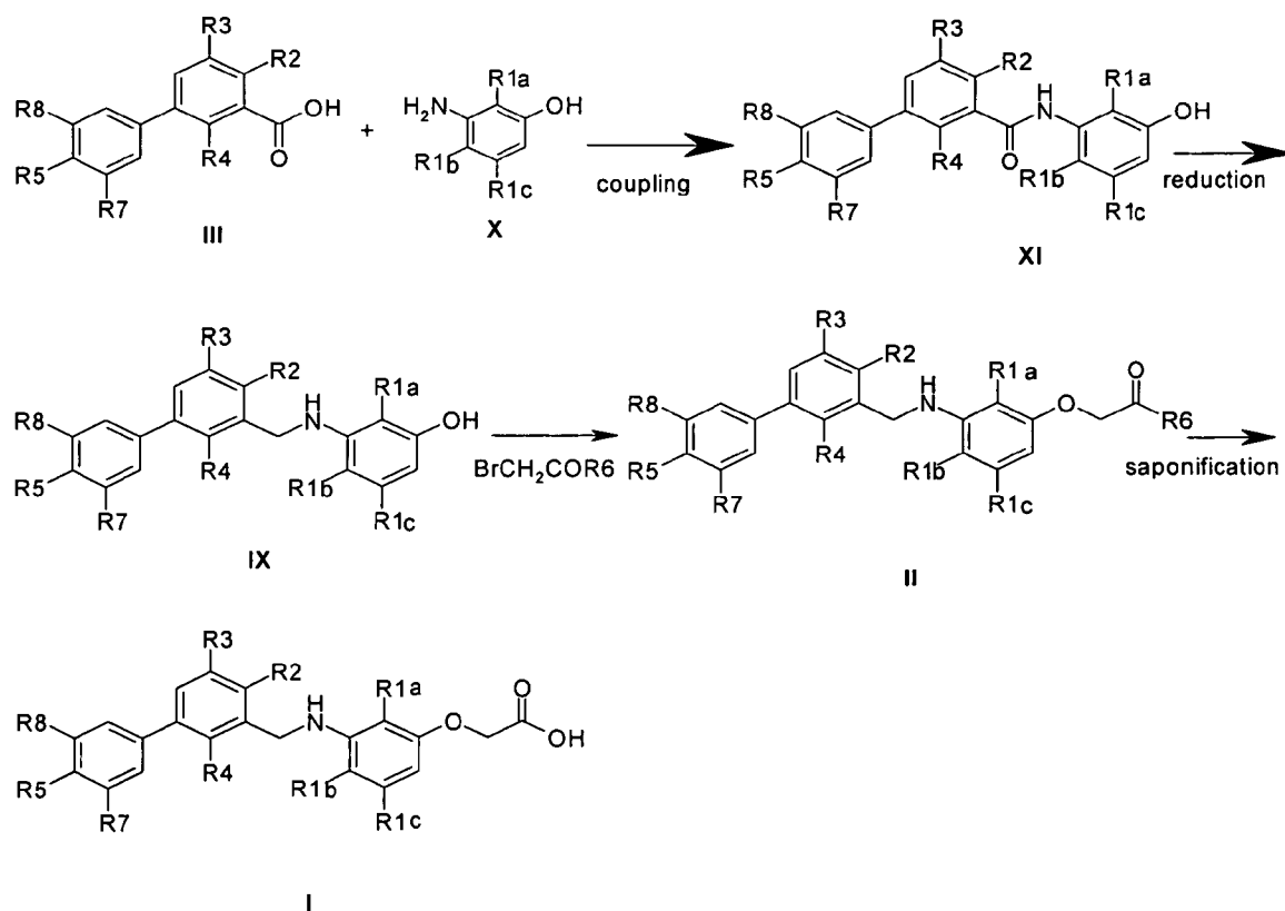
5 Scheme 3:
