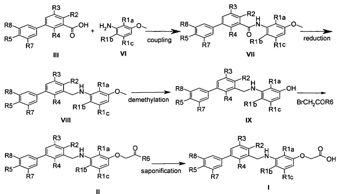
5 Scheme 3:
