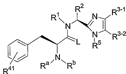
Formula (Ib)
