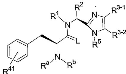
Formula (Ib)
