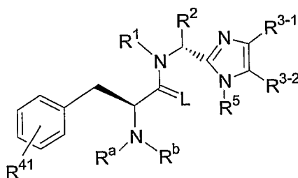
Formula (Ic)
