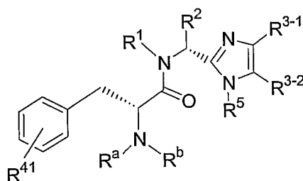
Formula (Ie)
