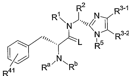
Formula (Ie)
