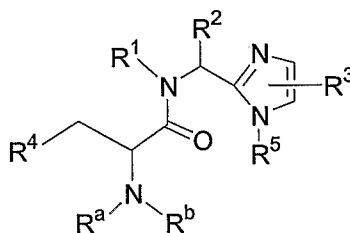
Formula (Ia)
