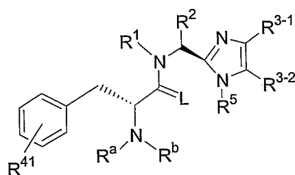
Formula (Id)
