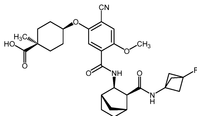
(Compound 6);
