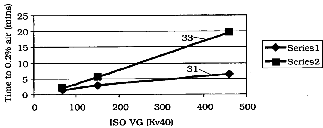
Fig X: ASTM D3427 (75C) results
