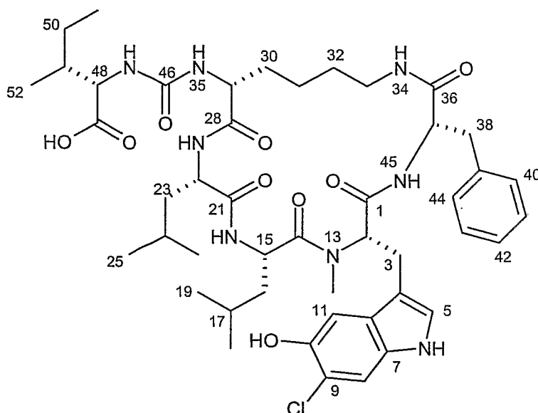
5 Table 9 1 H (600 MHz), 13 C (125 MHz), HMBC and COSY
