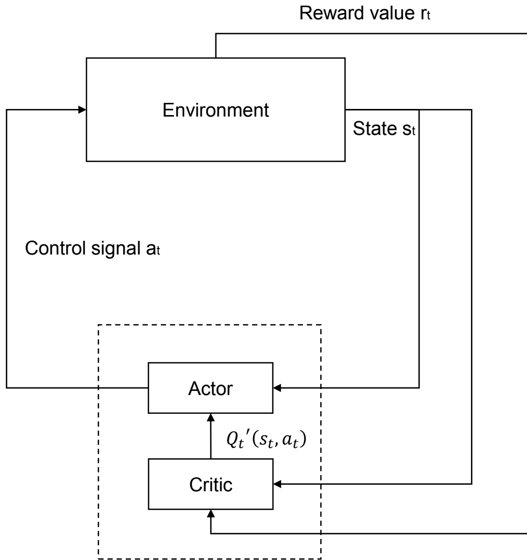
Deep Deterministic Policy Gradient (DDPG) network model
