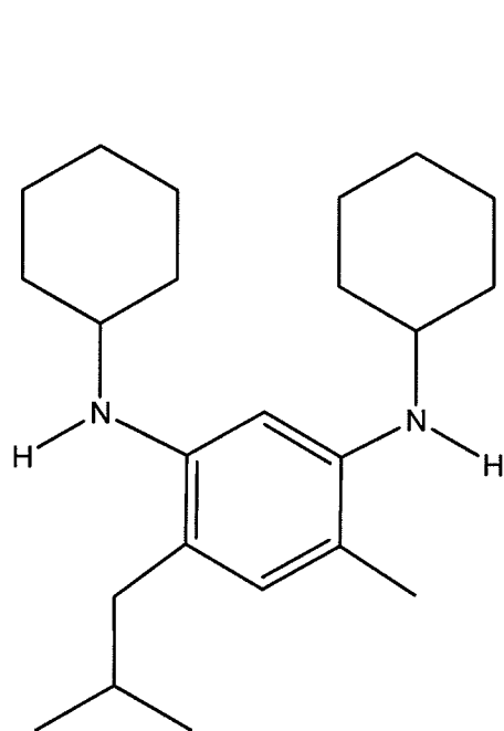
(XXVIII);
