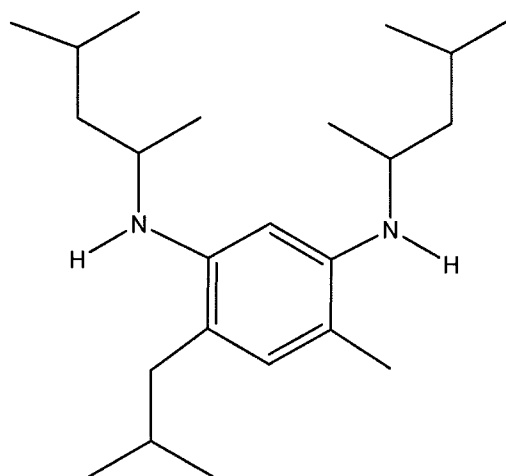
(XXIV);
