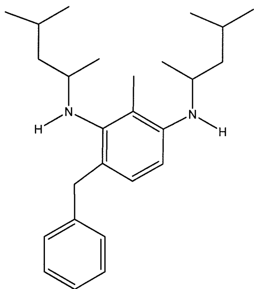
(XXXII);
