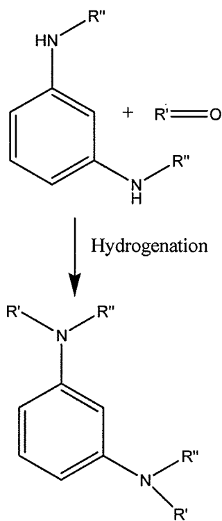
Expected Synthesis
