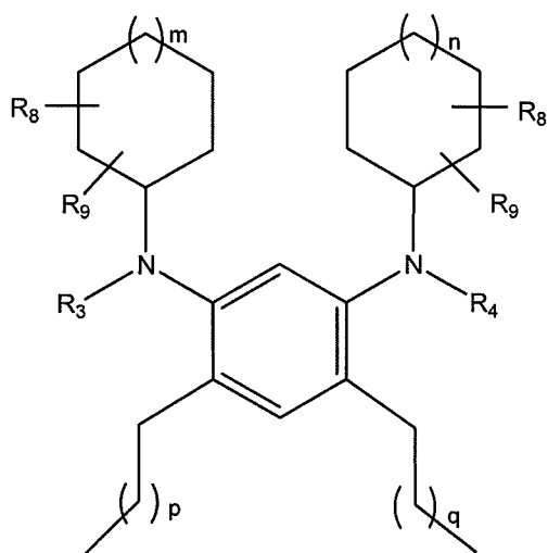
(VII) and
