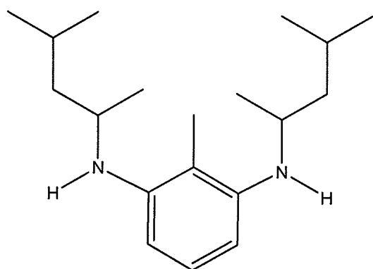
(XXX);
