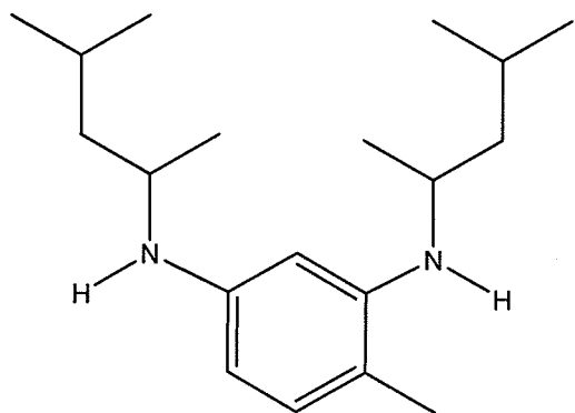
(XXIV);
