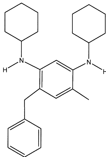
(XXVIII);
