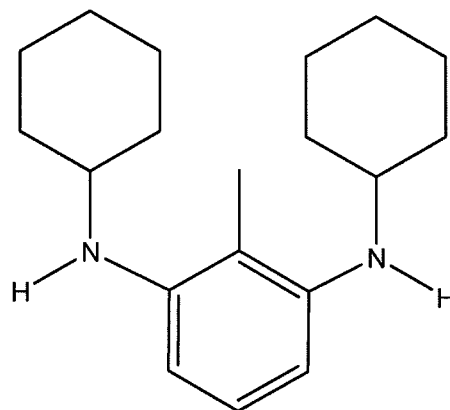
(XXXII);
