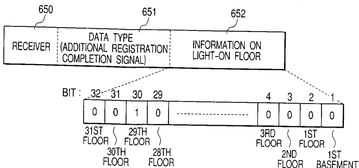
FORMAT OF REGISTERED FLOOR LIGHT-OFF SIGNAL
