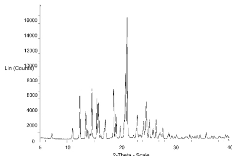
Figure 1: X-Ray Powder Diffraction Pattern for Form A of N-(1-(3-fluoropropyl)azetidin-3-yl)-6-((6S,8R)-8-methyl-7-(2,2,2-trifluoroethyl)-6,7,8,9-tetrahydro-3H-pyrazolo[4,3-f]isoquinolin-6-yl)pyridin-3-amine
