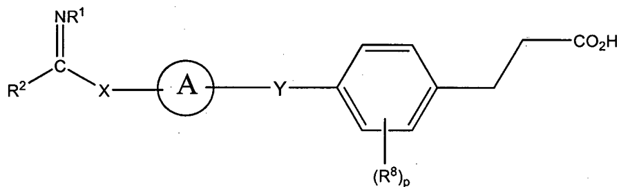
Formula (IVa)
