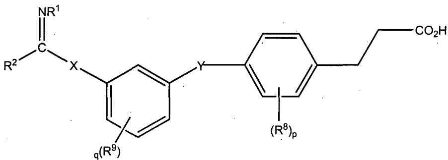
Formula (Vd)
