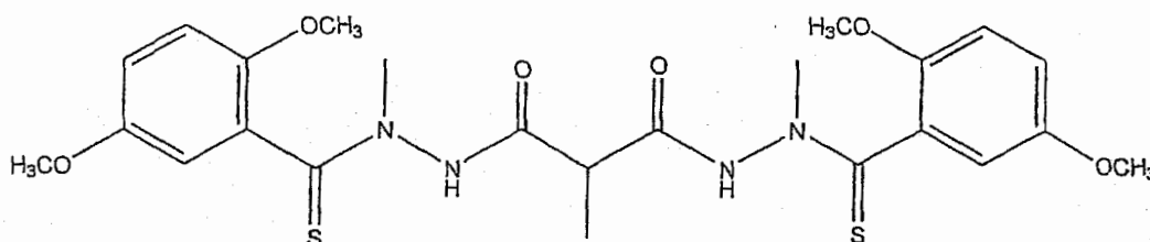
Compound (5)
