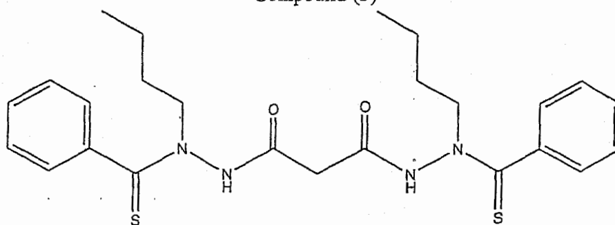
Compound (4)
