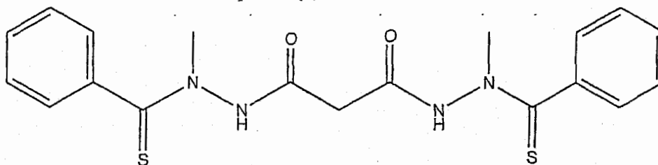
Compound (1)
