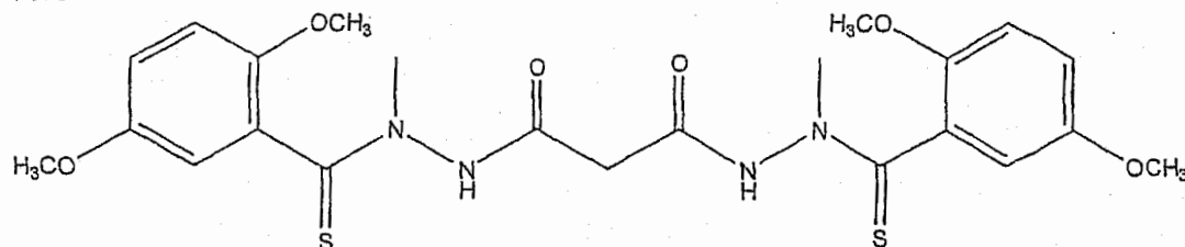
Compound (2)
