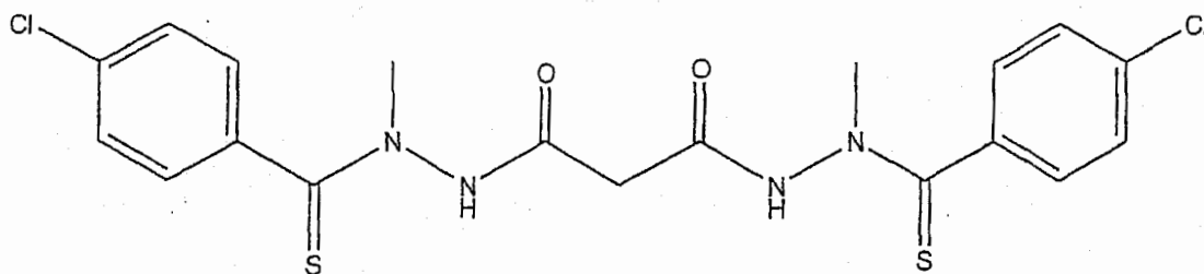
Compound (3)
