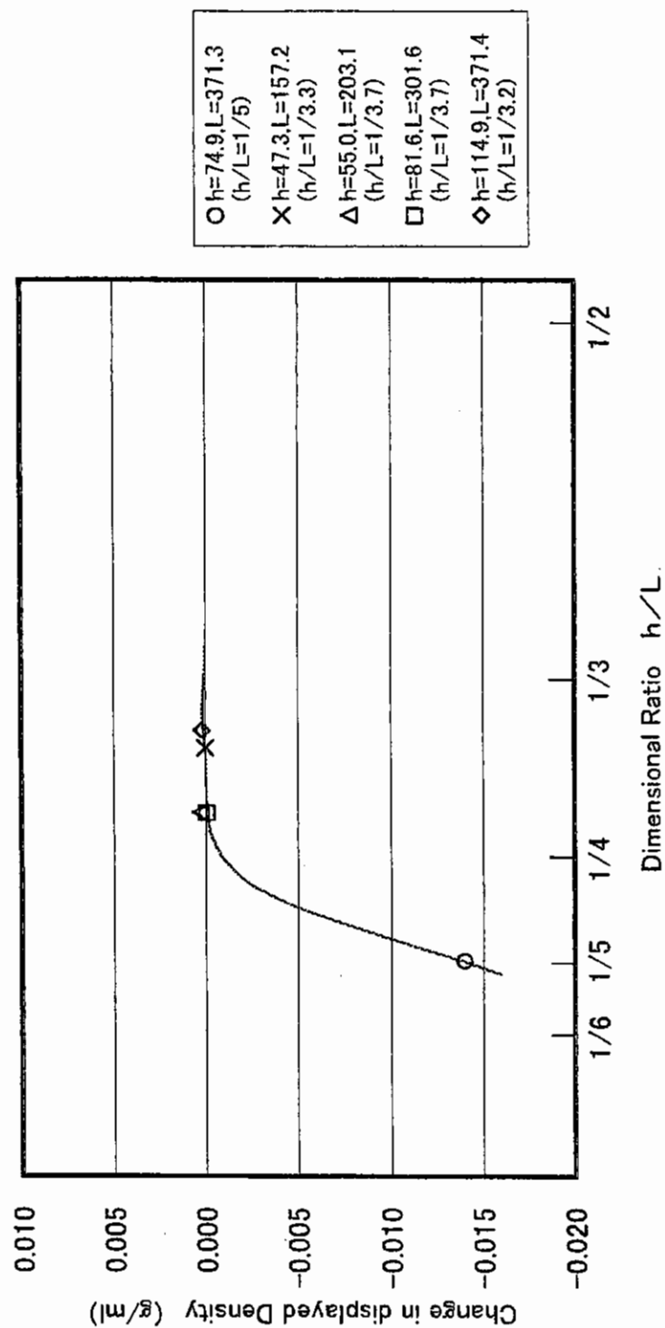
Fig.12 Change in displayed Density after Abrupt Temperature Change (Temperature Difference +110°C)
