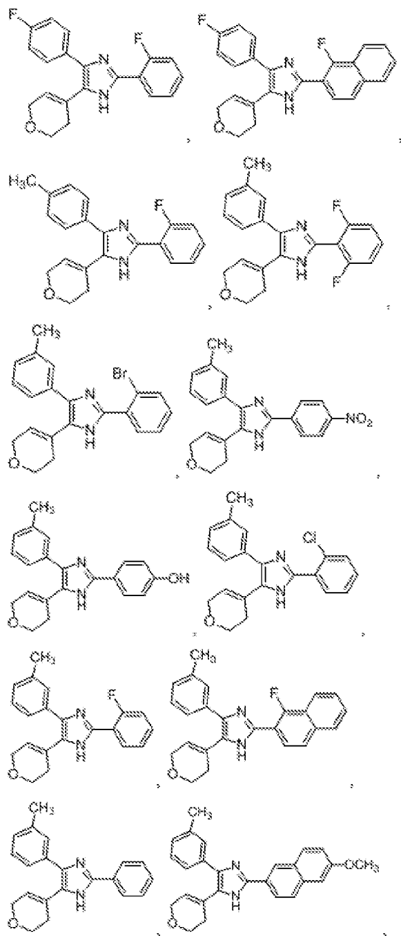
[Formula IIIc]
