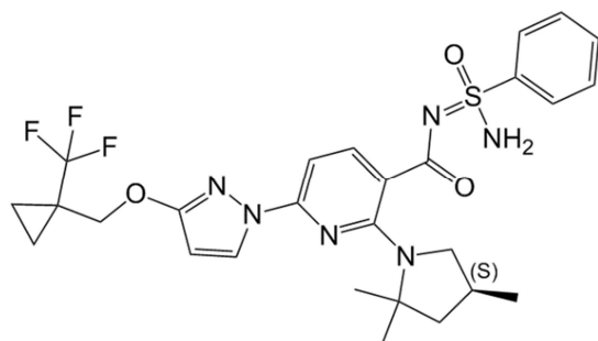
diastereomer 1
