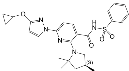
diastereomer 1
