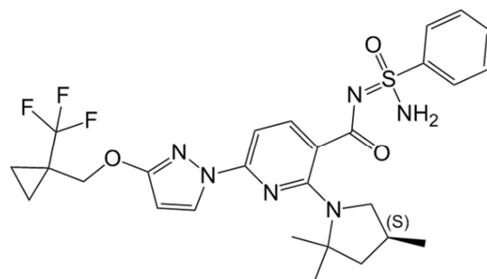
diastereomer 2
