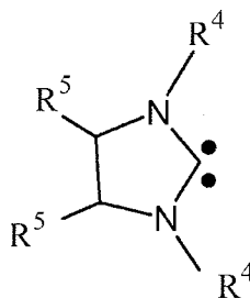
or Formula (IV)
