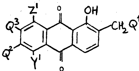
Formula (VII)
