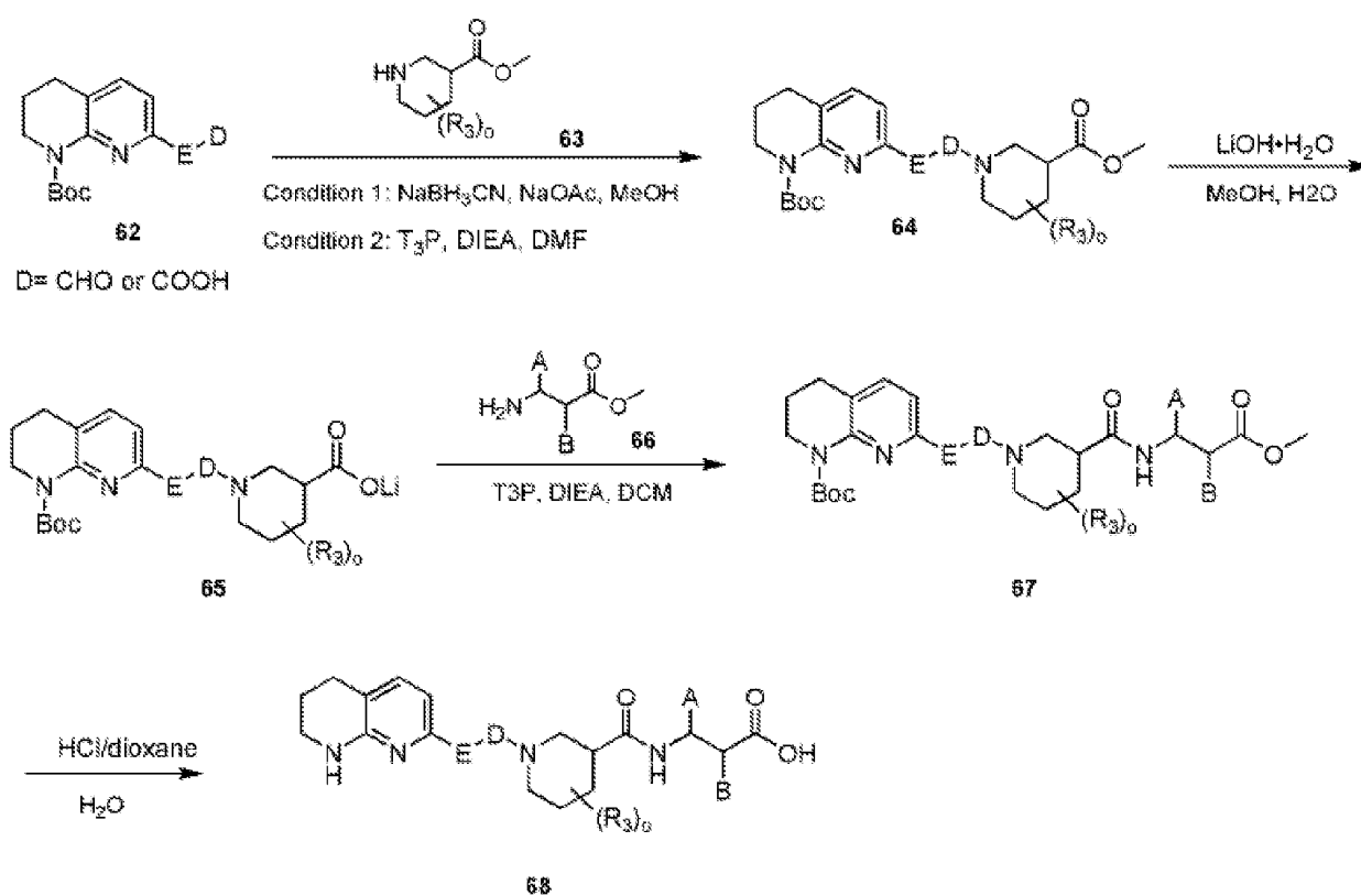
Scheme 14
