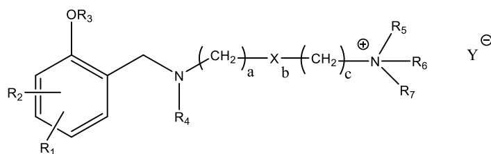
(Formula I)
