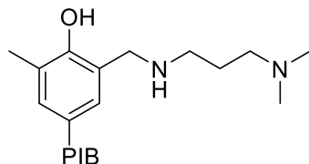
(Compound 10)
