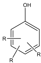
(Formula II)
