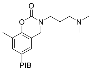
(Compound 3)
