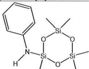
2-phenylamino-2,4,4,6,6-pentamethylcyclotrisiloxane
