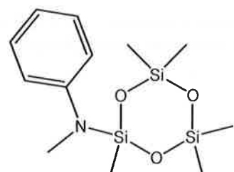
2-phenylmethylamino-2,4,4,6,6-pentamethylcyclotrisiloxane
