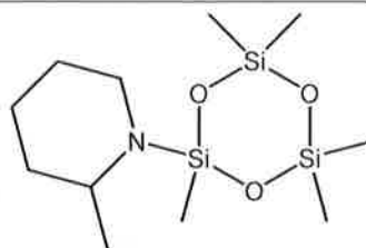
2-(2-methylpiperidino)-2,4,4,6,6-pentamethylcyclotrisiloxane
