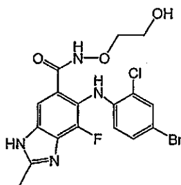
6-(4-Bromo-2-chloro-phenylamino)-7-fluoro-2-methyl-3H-benzimidazole-5-carboxylic acid (2-hydroxy-ethoxy)-amide (10ii)
