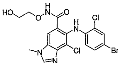
6-(4-Bromo-2-chloro-phenylamino)-7-chloro-3-methyl-3H-benzoimidazole-5-carboxylic acid (2-hydroxy-ethoxy)-amide (10cc)
