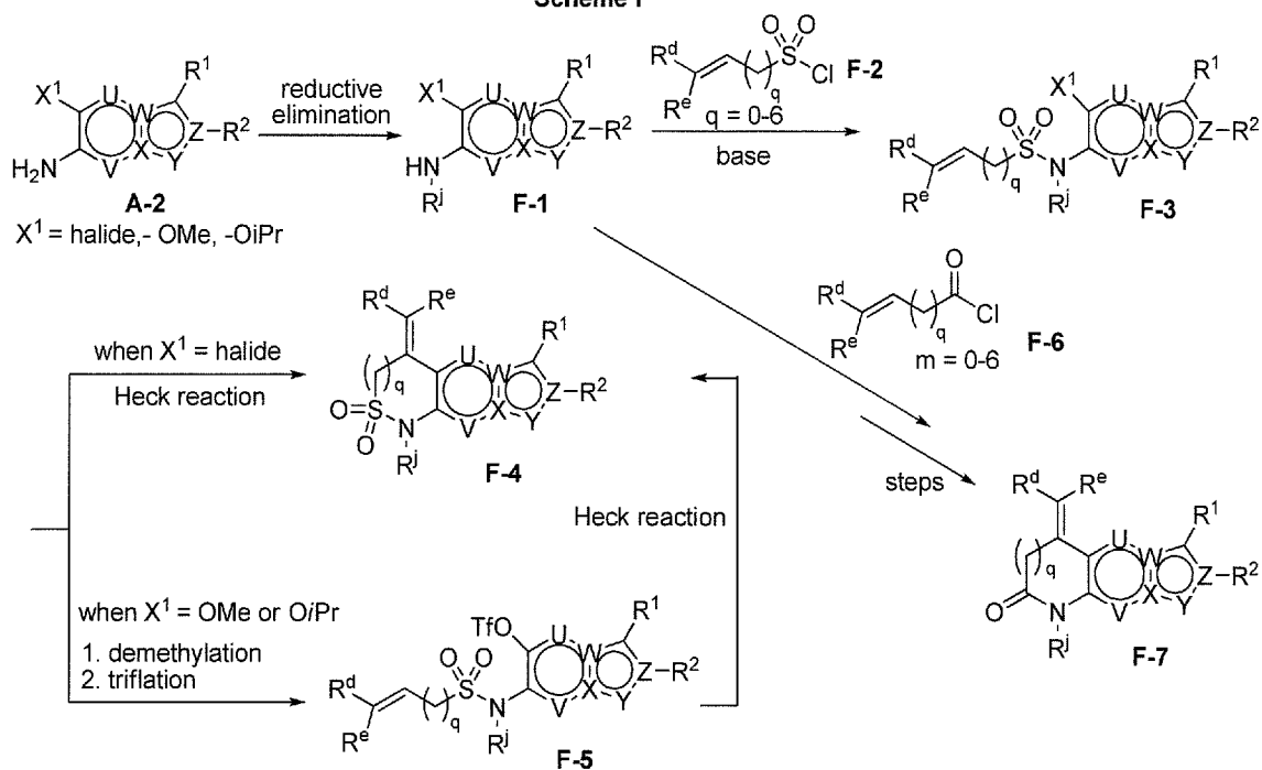
Scheme F
