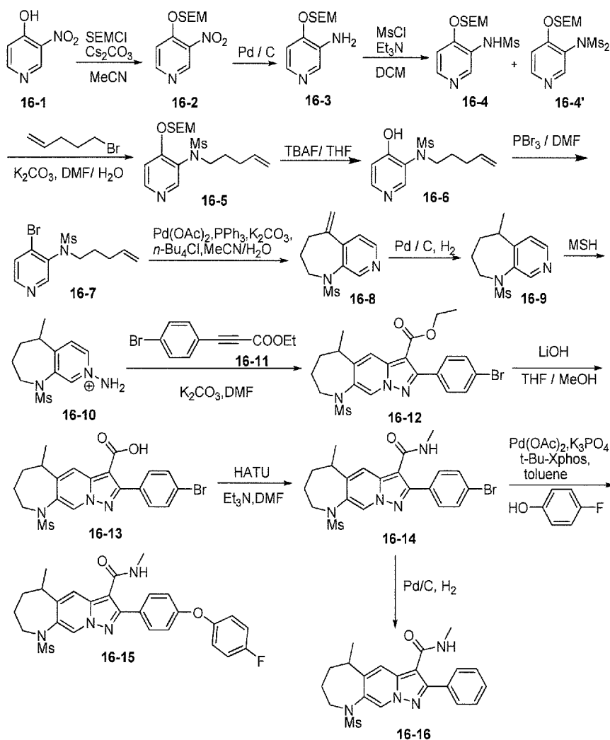
Scheme 16
