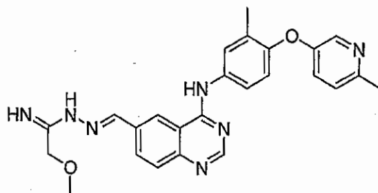
(E)-N-(4-(3-Methyl-4-(6-methylpyridin-3-yloxy)phenylamino)quinazolin-6-yl)methyleneamino-2-methoxyacetamide
