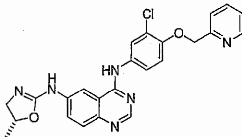
(R)-N4-[3-Chloro-4-(pyridin-2-ylmethoxy)-phenyl]-N6-(5-methyl-4,5-dihydro-oxazol-2-yl)-quinazoline-4,6-diamine
