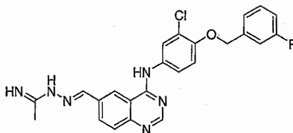
(E)-N-((4-(4-(3-Fluorobenzoyloxy)-3-chlorophenylamino)-quinazolin-6-yl)-methyleneamino)-acetamide
