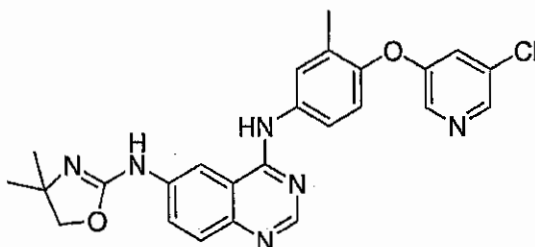
N4-[4-(5-Chloropyridin-3-yloxy)-3-methyl-phenyl]-N6-(4,4-dimethyl-4,5-dihydro-oxazol-2-yl)-quinazoline-4,6-diamine
