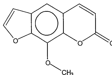
8-Methoxypsoralen
