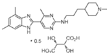
2.1 Polymorph A
