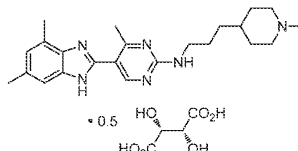
2.2 Polymorph B
