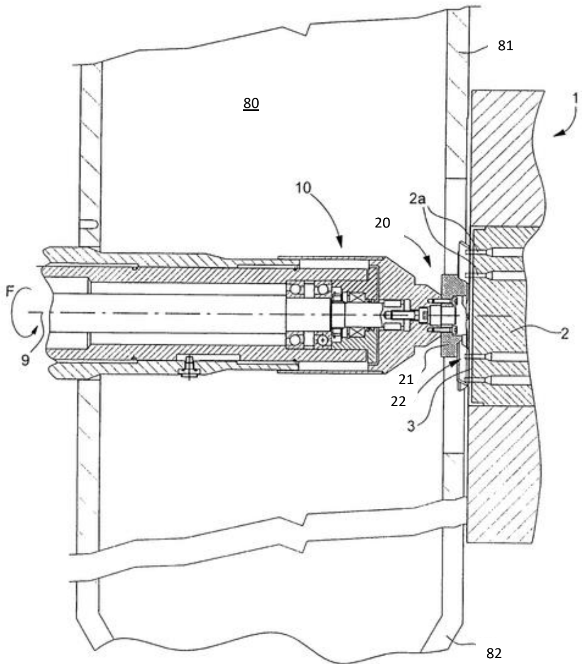
FIGURE 9 (prior art)
