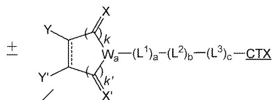
linker-cytotoxin conjugate
