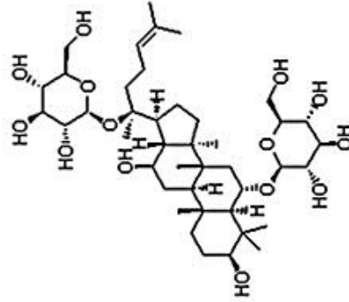
Ginsenoside Rc
