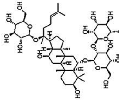
Ginsenoside Rb2
