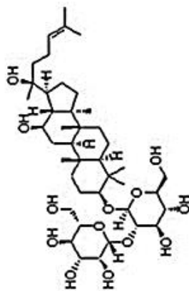
Ginsenoside Rb1
