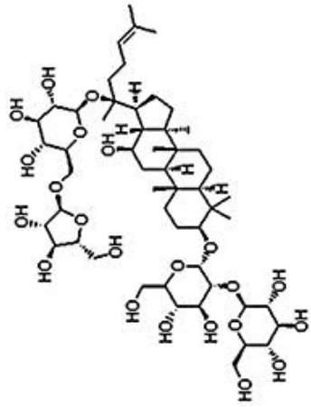
Ginsenoside Rc
