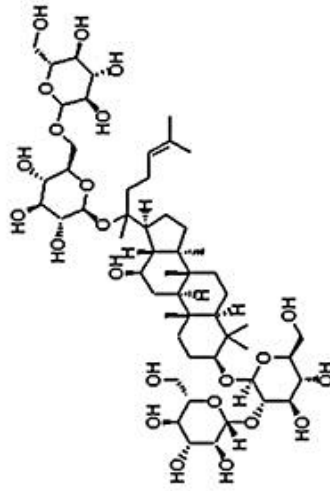
Ginsenoside Rb2
