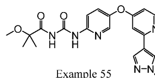
Example 55
