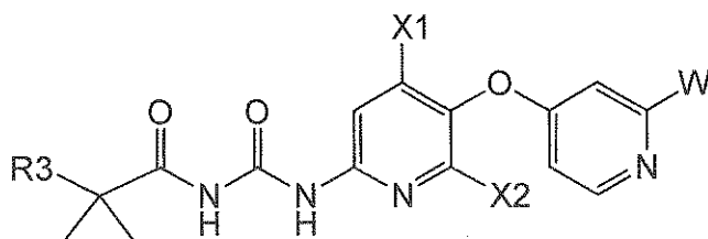
Formula Ib
