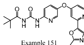
Example 151
