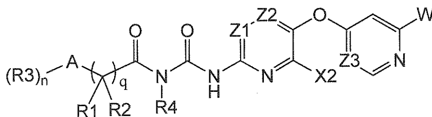
Formula I
