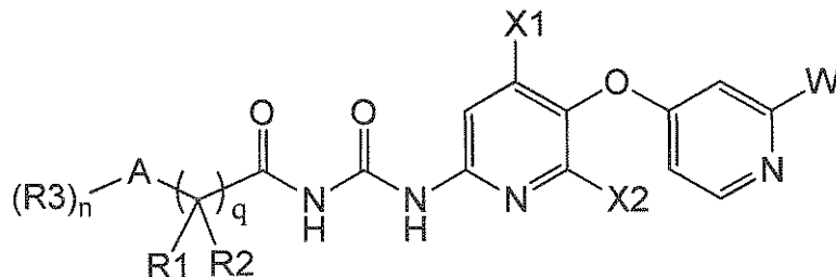
Formula Ia
