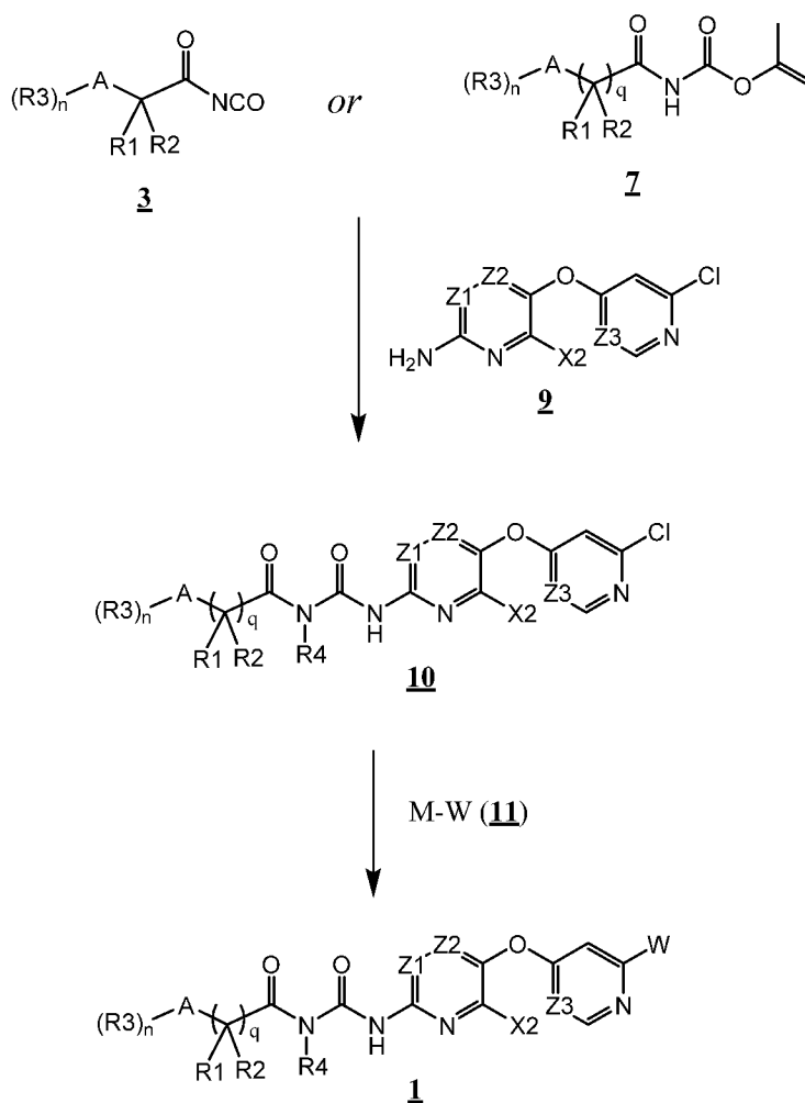
Scheme 2
