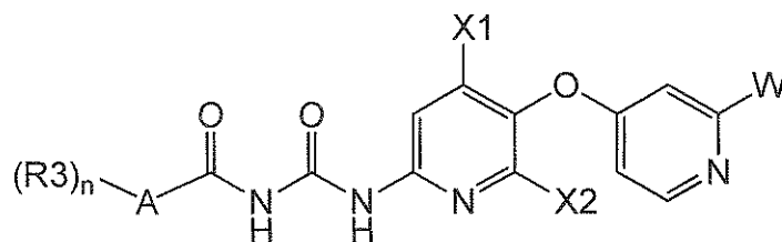
Formula Id
