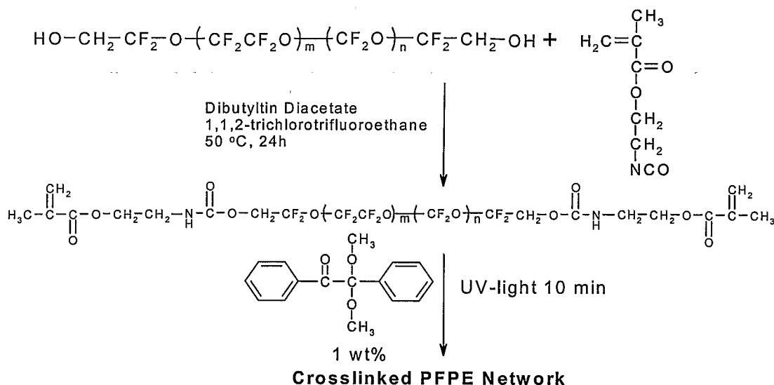
Scheme 1. Synthesis and Photocuring of Functionalized Perfluoropolyethers.
