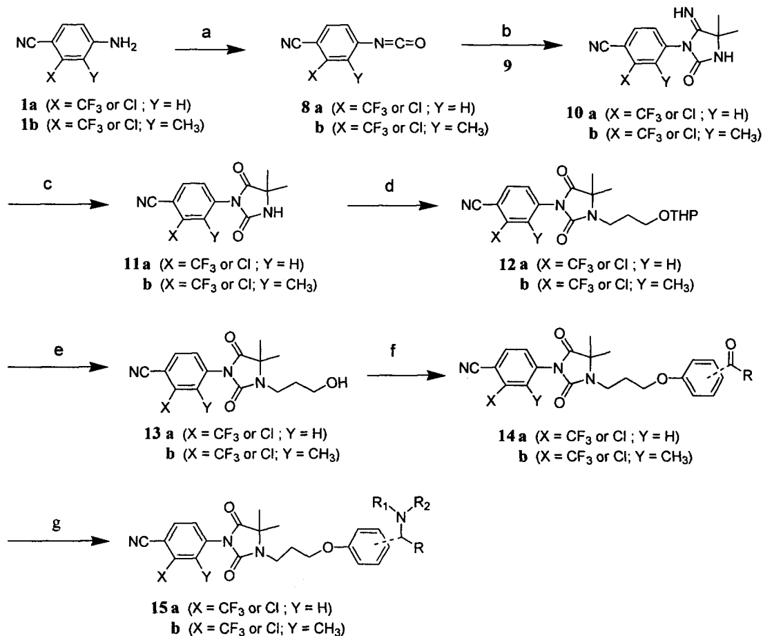
Scheme 2
