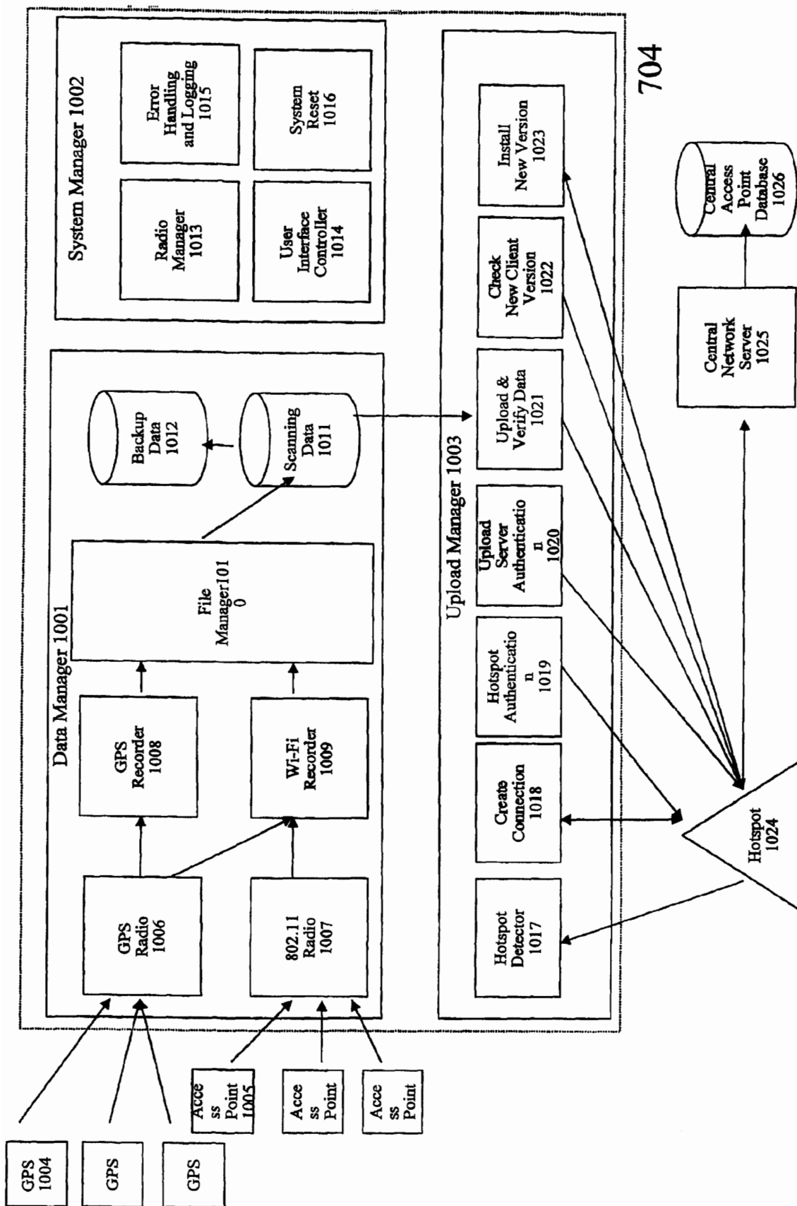
Figure 10: Scanning Client
