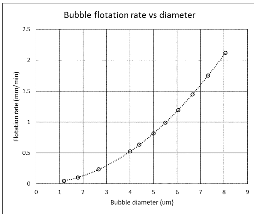
Figure 3: Flotation rate vs bubble size.
