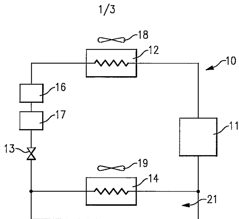
FIG. 1 Prior Art
