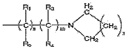
aminoalkyls
