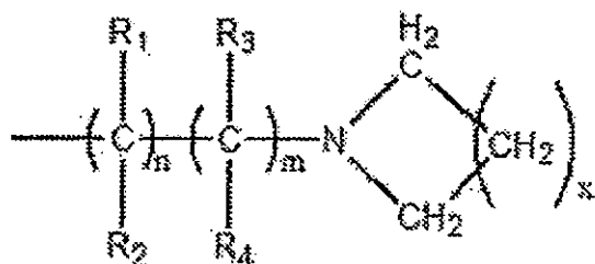
aminoalkyls
