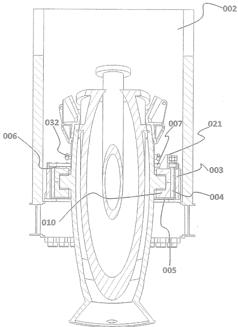
SECTION C-C
