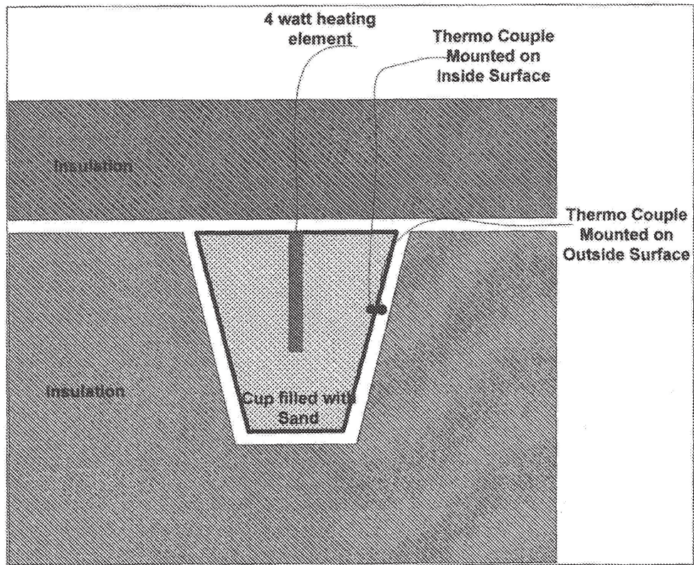
Thermal Resistance Test Assembly
