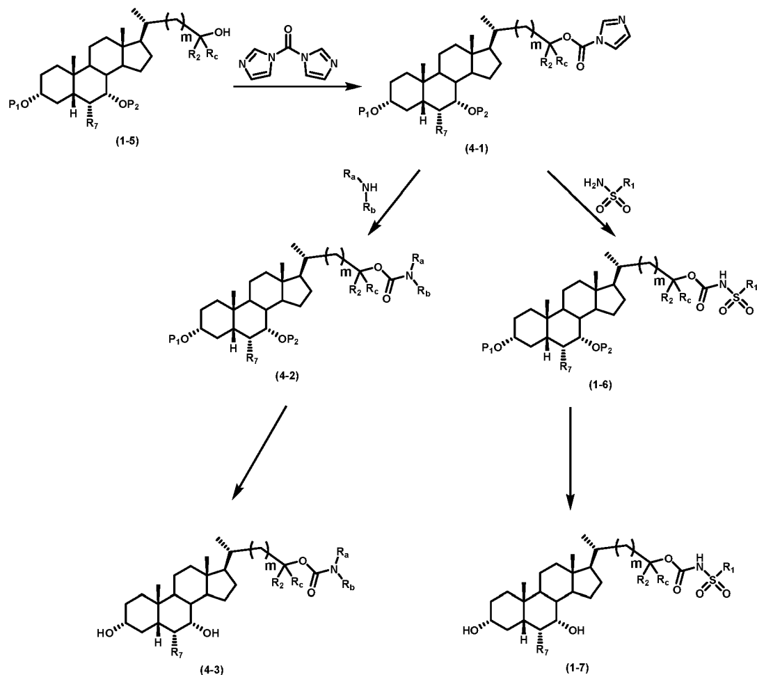
Scheme 4
