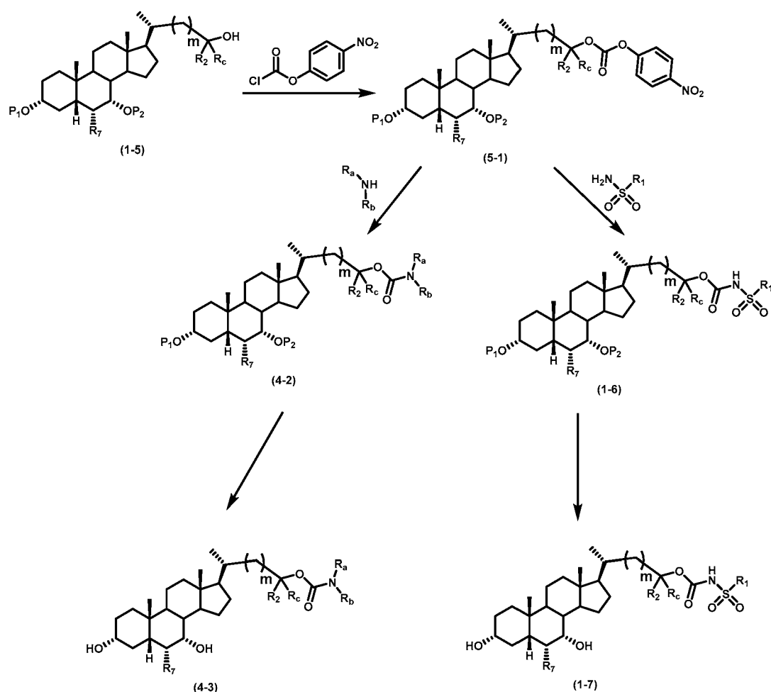
Scheme 5
