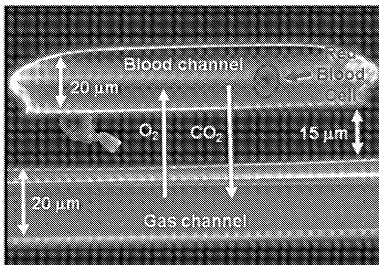
Microchannel Artificial Lung
