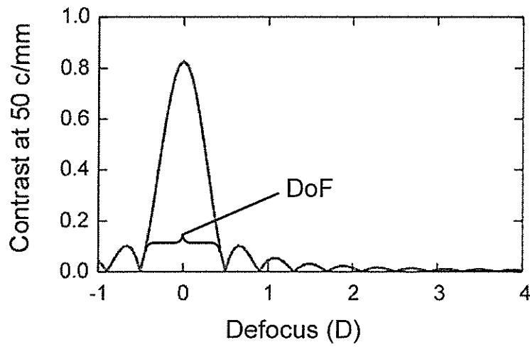
FIG. 2A IOL Eliminates Aberration
