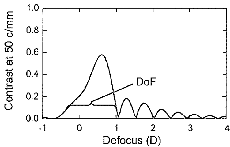
FIG. 2C Aspheric IOL Adds Aberration
