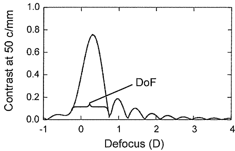
FIG. 2B Spherical IOL
